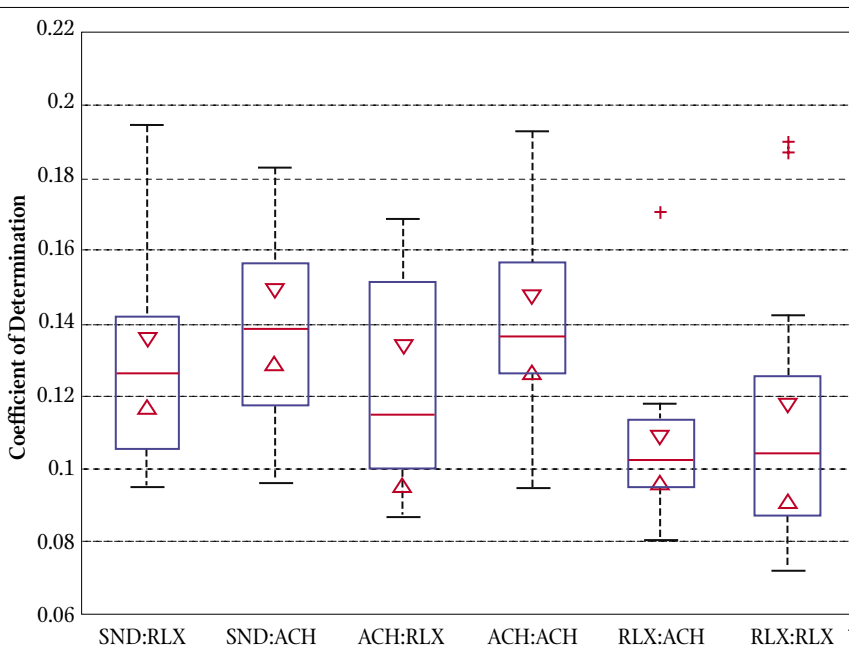
FIGURE 7 Mean of Average Coefficient of Determination between Participants by Mode
